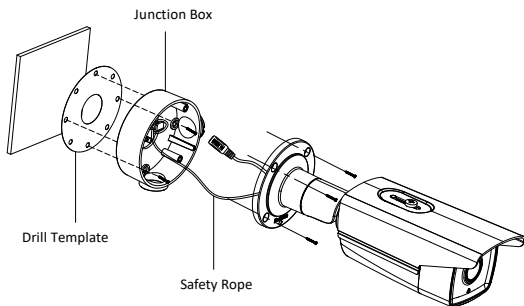
Figure 2-8 Installation with a Junction Box
