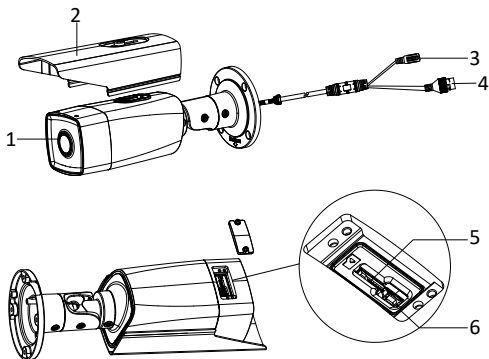
Figure 1-1 Overview of camera
