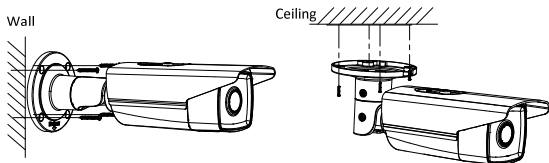
Figure 2-4 Install the Camera
