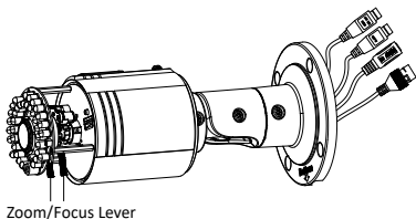
Figure 2-9 Zoom and Focus Adjustment
