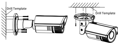
Figure 2-6 Secure the Camera
