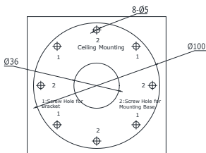
Figure 2-5 Drilling Holes in the Wall/Ceiling
