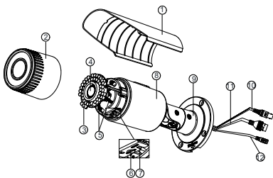
Figure 1-1 Overview of Camera
